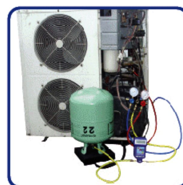
Charging for A/C system 空调加注示冷媒意图
